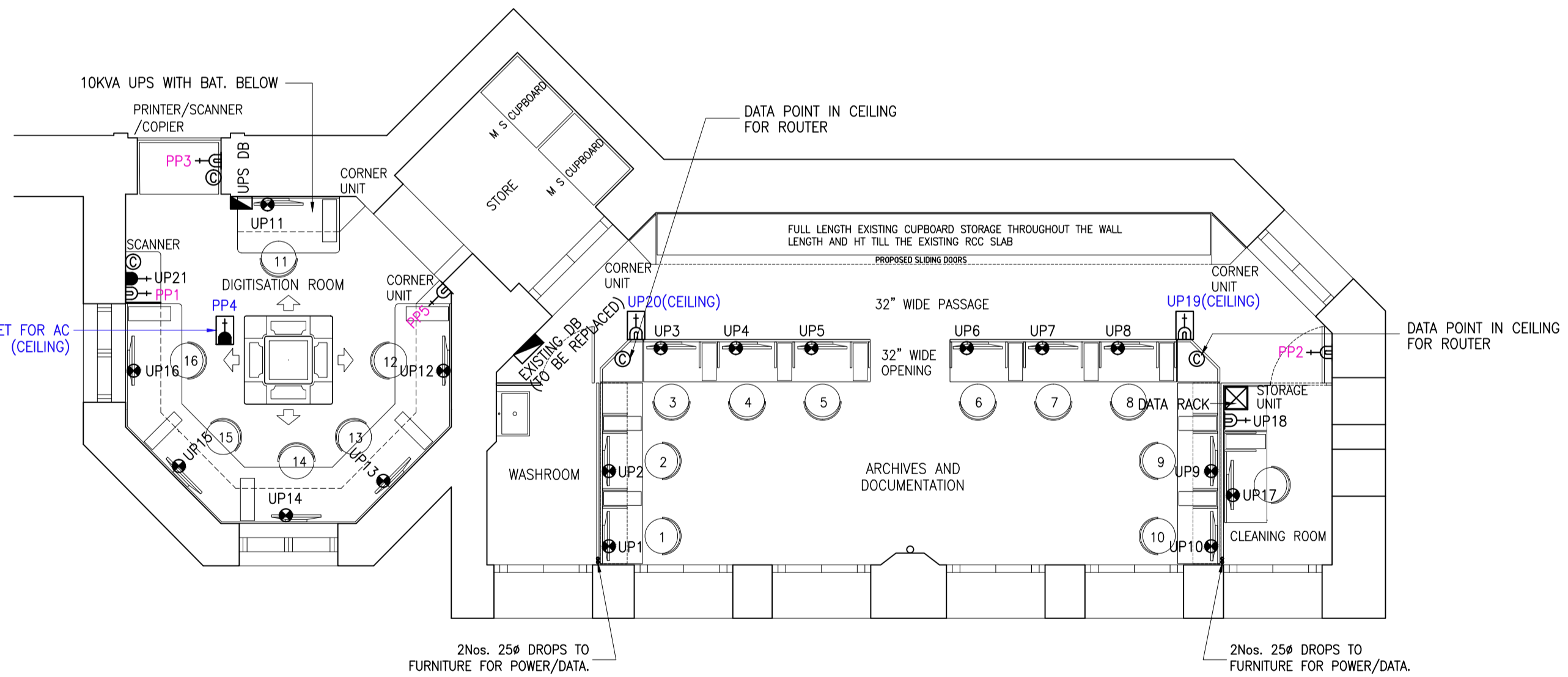
POWER & ELV LAYOUT
