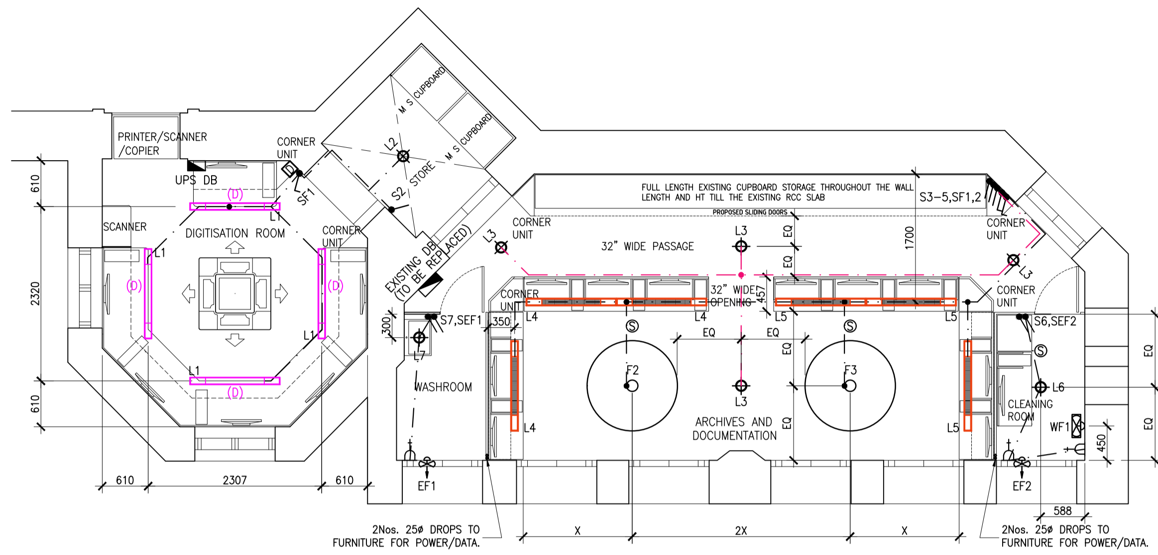
LIGHTING LAYOUT
