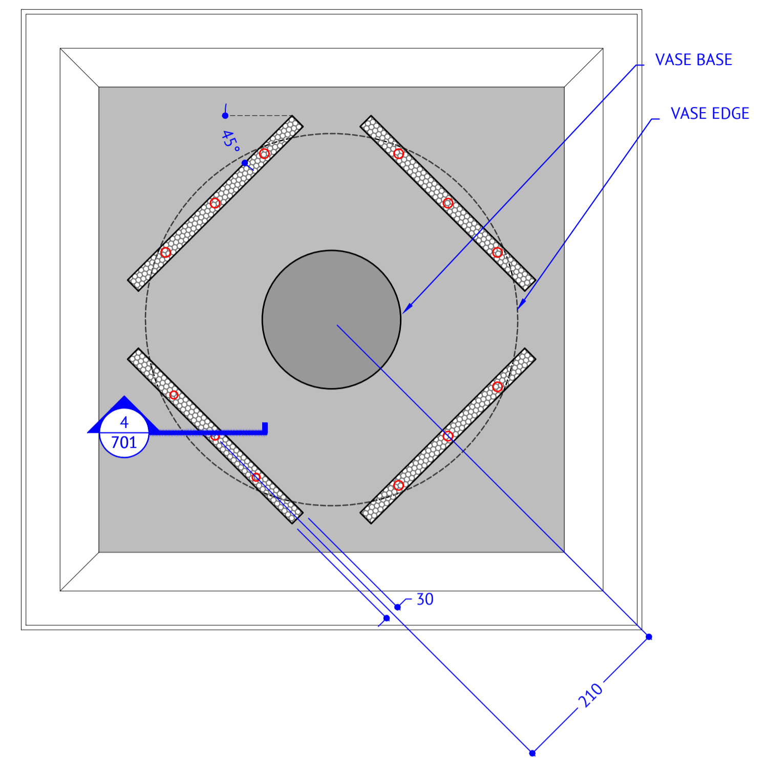
3 PLAN FOR VASE 2 1:5
