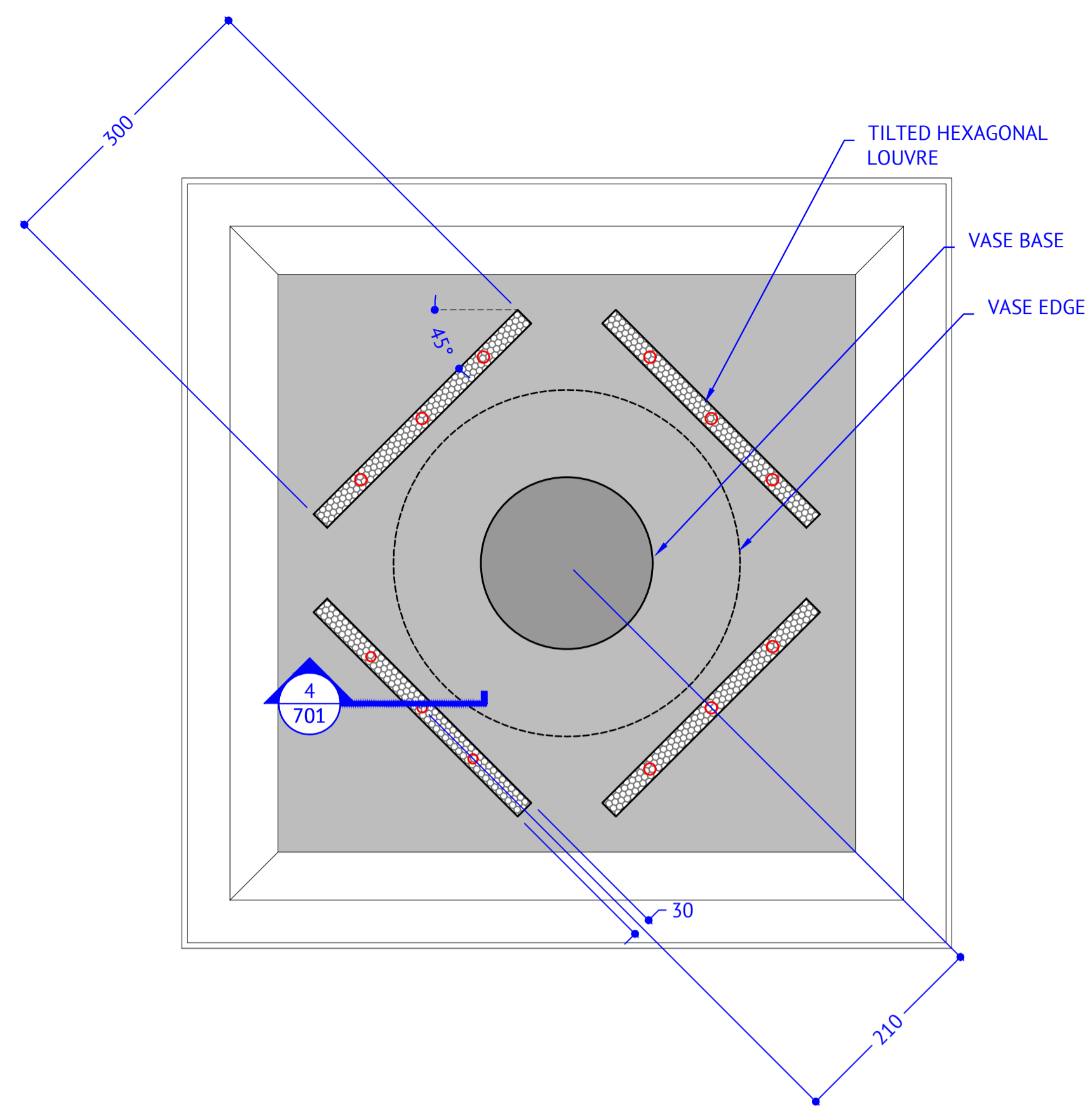
2 PLAN FOR VASE 1 1:5
