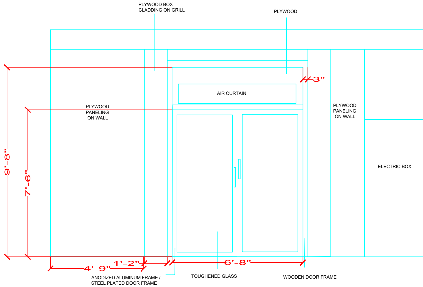
EAST WING FIRST FLOOR DOOR Date 14/ 12/ 2022
