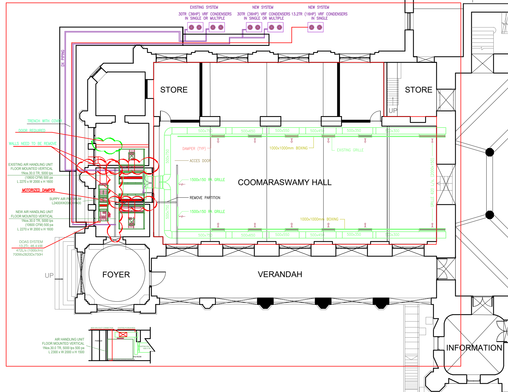
MEZZANINE PLAN
